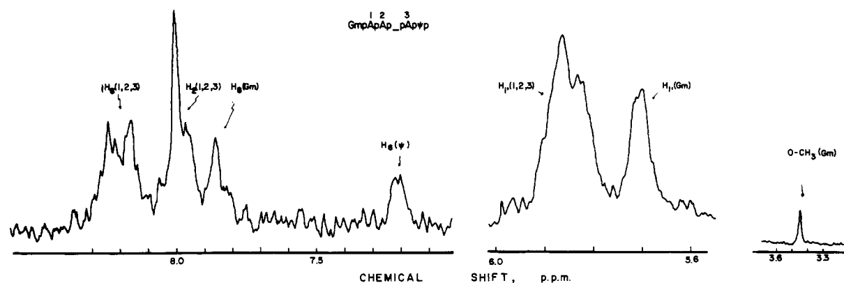
FIGURE 4: A 250-MHz ^1\text{H} NMR spectrum of GmpApAp—pApψp recorded by Fourier transform mode (160 pulses) at 32° together with all the assignments.
