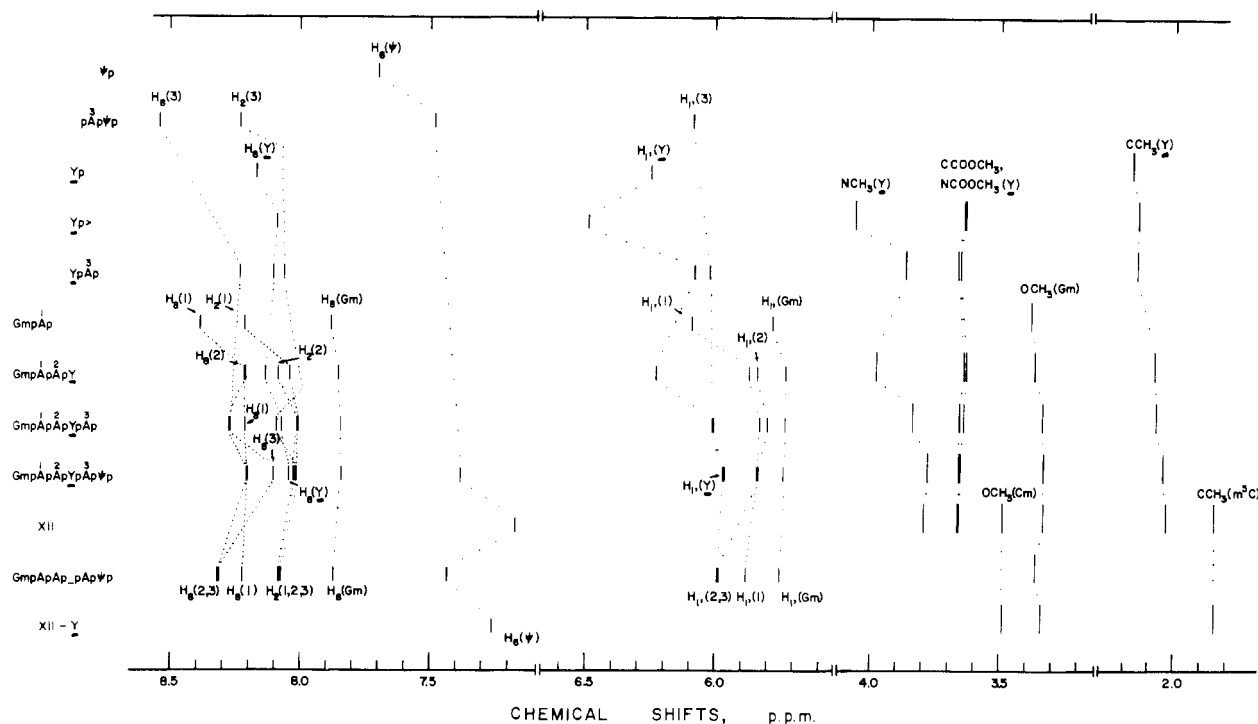
FIGURE 2: Assignments of the proton resonances in 12 compounds by systematic "incremental assignment". The ^1\text{H} NMR spectra were recorded at 63^\circ with the quantities of the compounds in Table I dissolved in 0.3 ml of \text{D}_2\text{O} , containing 0.01 M phosphate buffer (pD 7) and 5 \times 10^{-5} M EDTA. XII and XII-Y are dodecamer and dodecamer-Y.
