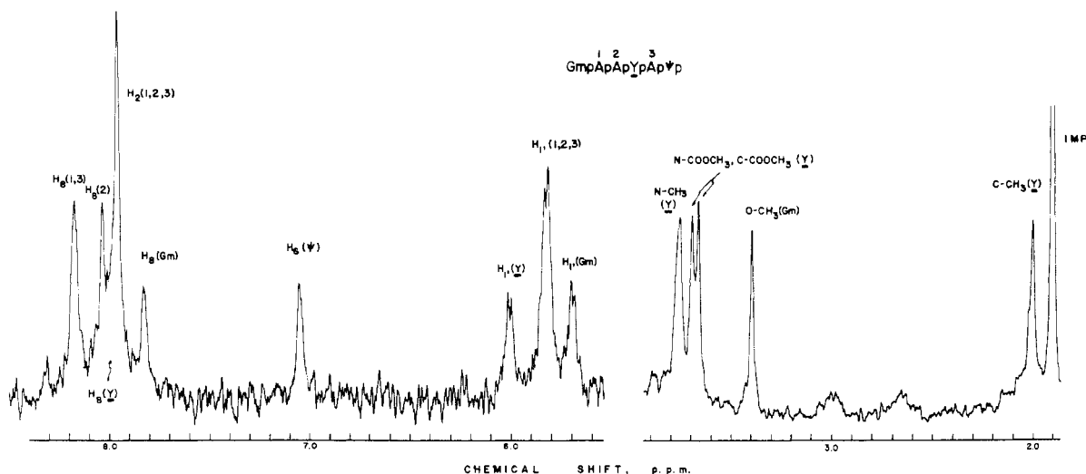
FIGURE 3: A 250-MHz ^1\text{H} NMR spectrum of GmpApApYpApΨp recorded by continuous wave mode at 32^\circ together with all the assignments. A signal for impurity was found at \sim 1.9 ppm.
